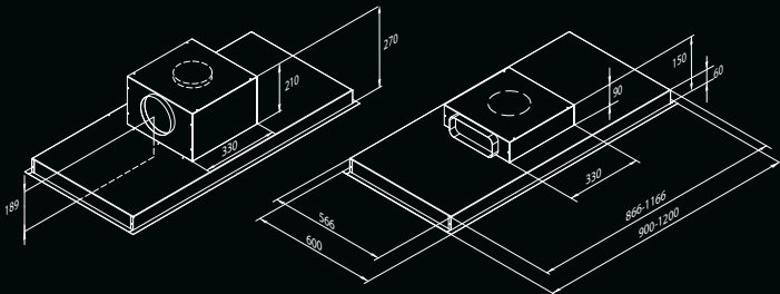
With Premium+ motor Without motor (for remote motors)
