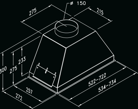
This model is a cut-out canopy extractor Minimum distance from induction hob: 500mm
