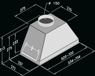
This model is a cut-out canopy extractor Minimum distance from induction hob: 500mm
