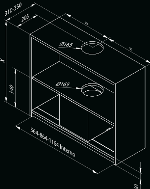
This model is a fully integrated canopy extractor Minimum distance from induction hob: 500mm
